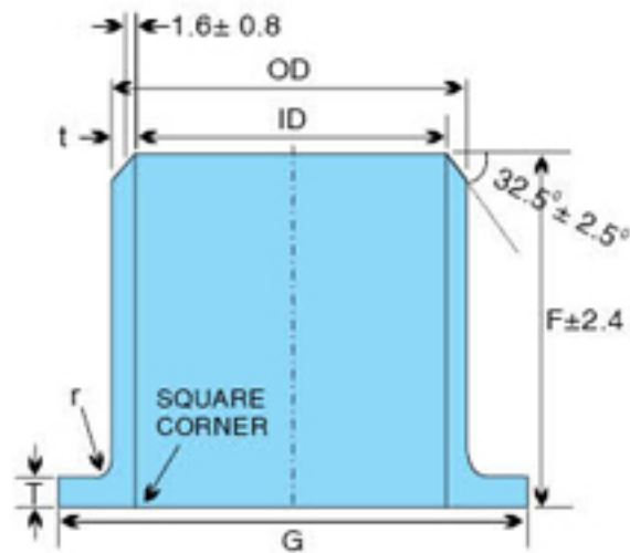
STUB END
